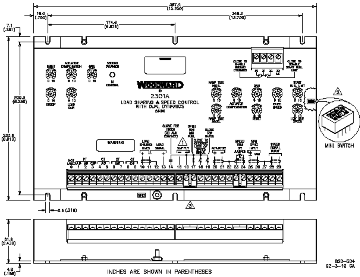
Outline Drawing of 2301A with Dual Dynamics (Do not use for construction)
