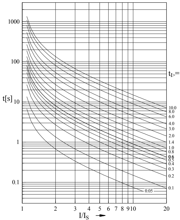
Figure 7.2: Very inverse tripping characteristic
