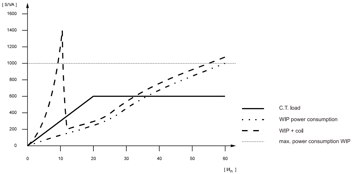
Figure 4.9: WIP1 - power consumption
