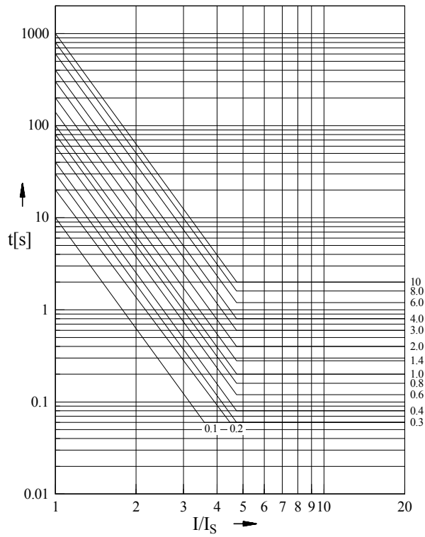
Figure 7.11: x^4 - tripping characteristic
