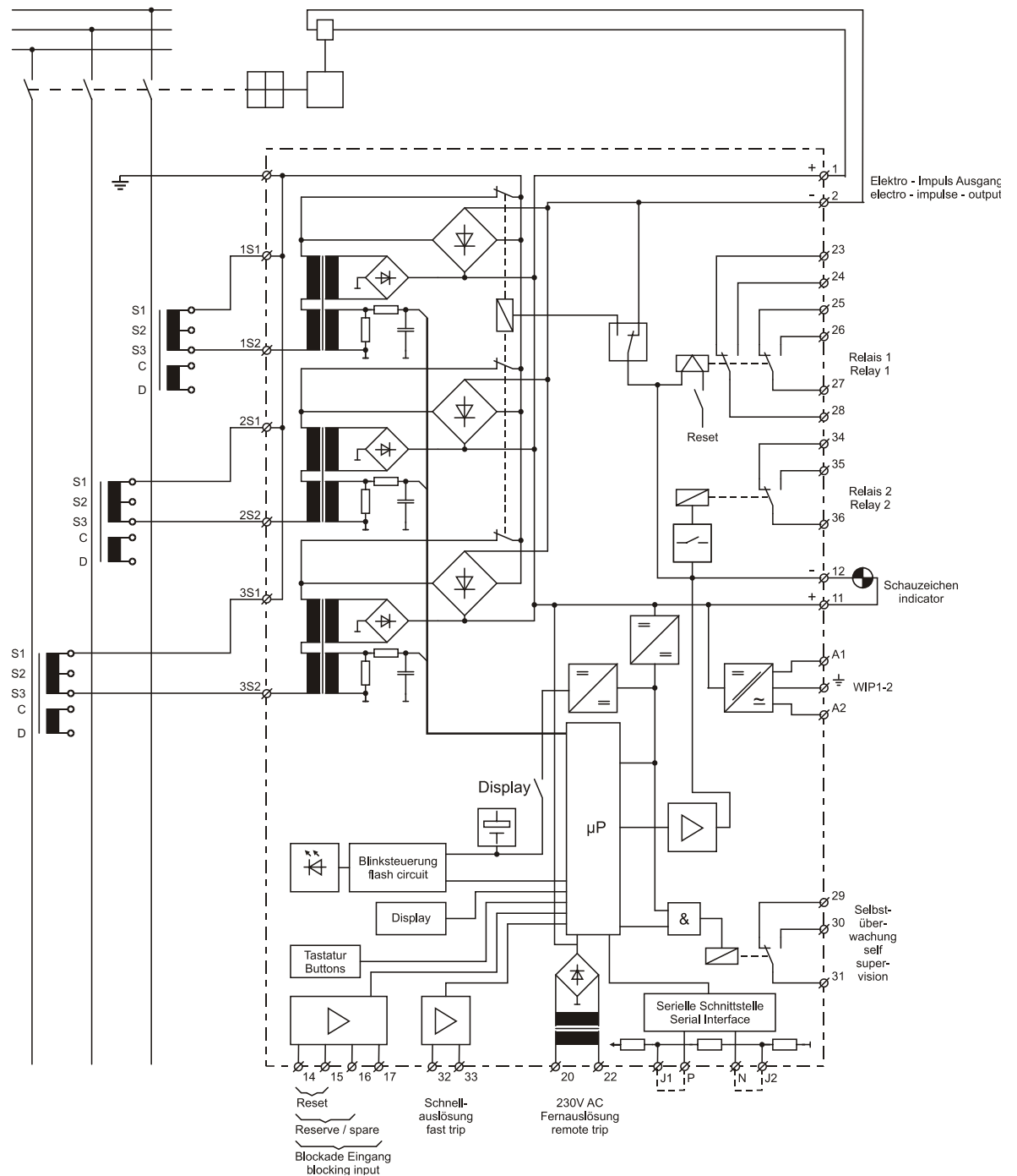
Figure 3.3: Block diagram WIP1-11 (only phase current measuring)
