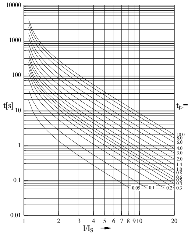
Figure 7.3: Extremely inverse tripping characteristic
