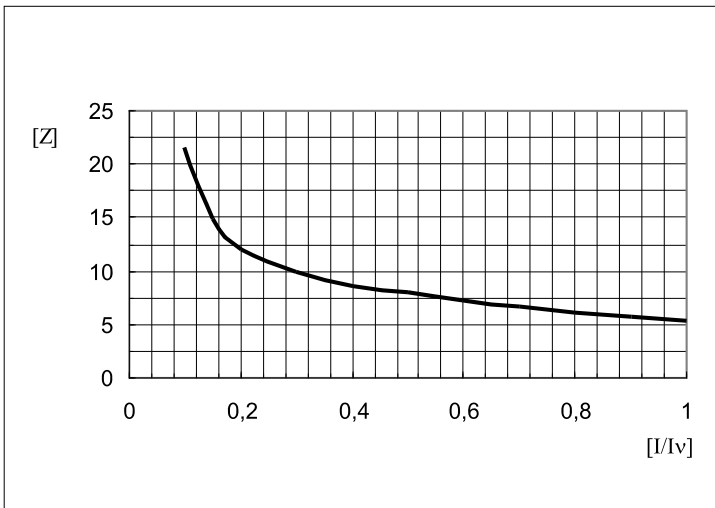
Figure 4.7: Diagram 1: WIP1 impedance curve for the range: 0.1A to 1A
