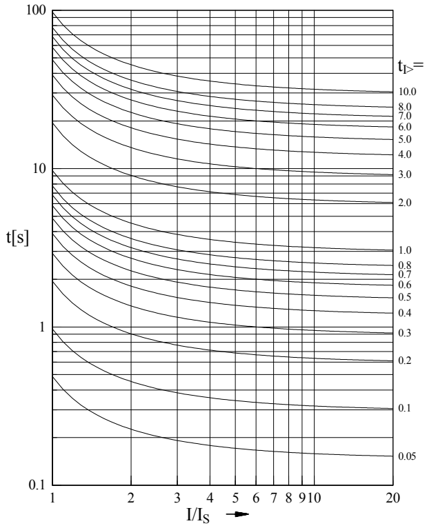
Figure 7.5: Ri-Inverse
