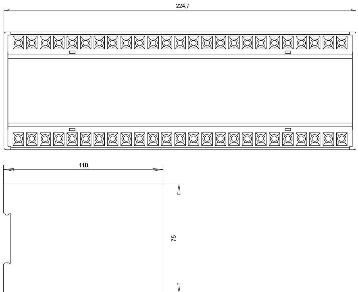
Figure 7.14: Dimensions WIP1 in mm
