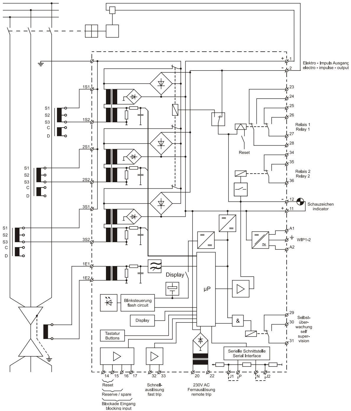
Figure 3.4: Block diagram WIP1-I1-E1 with earth fault detection via C.T. cable type
