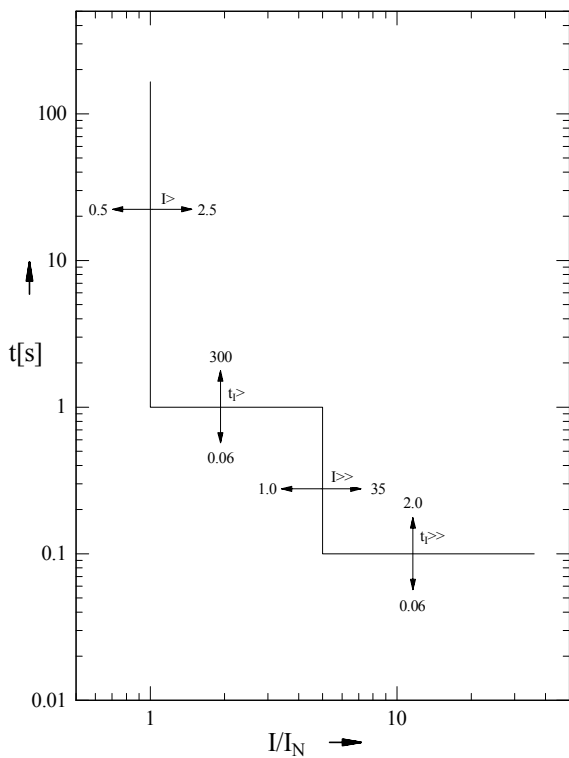
Figure 7.6: Definite time tripping characteristic
