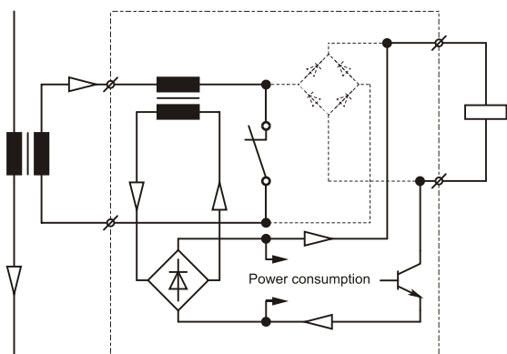
Figure 4.4: Tripping via self-supply as from 12 \times I_n
