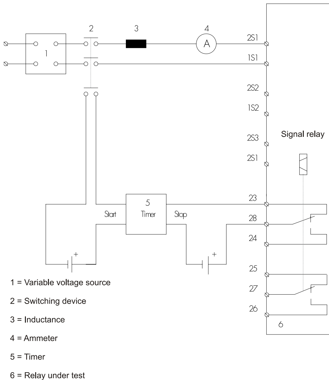
Figure 6.1: Test circuit
