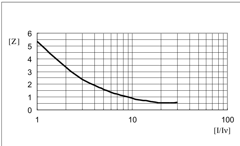
Figure 4.8: Diagram 2: WIP1 impedance curve for the range: 1 A to 30 A
