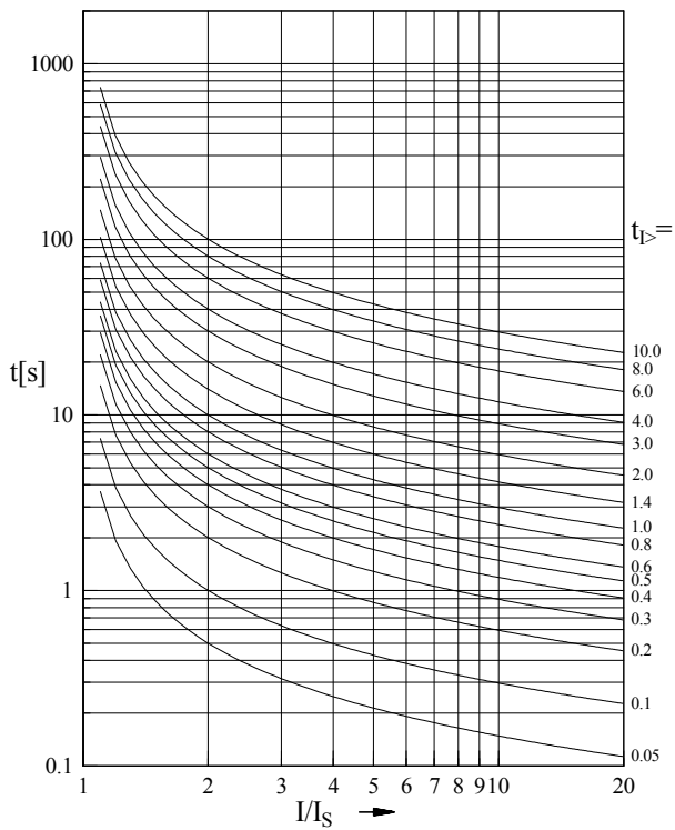
Figure 7.1: Normal inverse tripping characteristic
