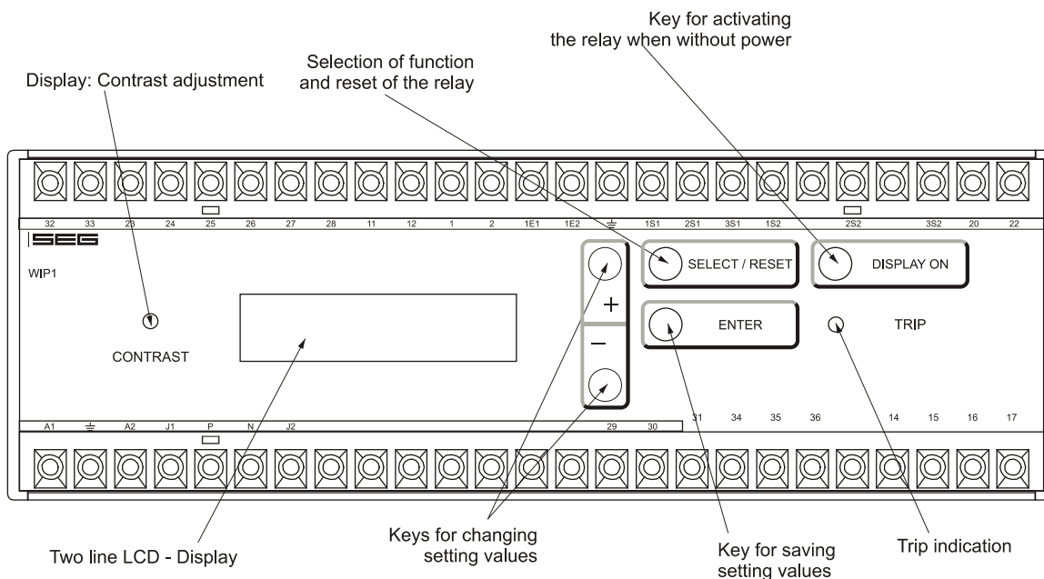
Figure 4.1: Front plate of WIP1
