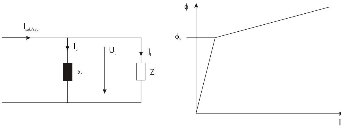
Figure 4.6: Circuit diagram of the secondary C.T. side and magnetizing curve
