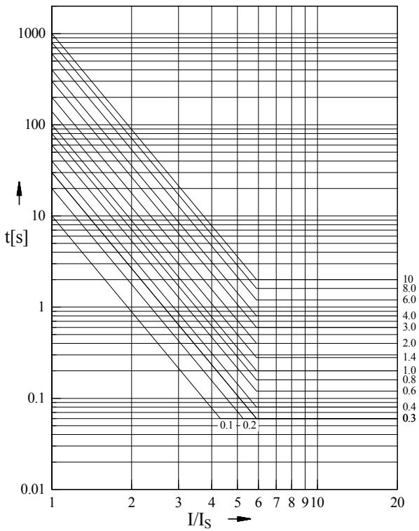
Figure 7.10: x^{3.5} - tripping characteristic
