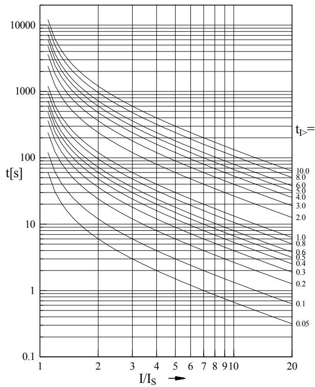
Figure 7.4: Long Time Inverse
