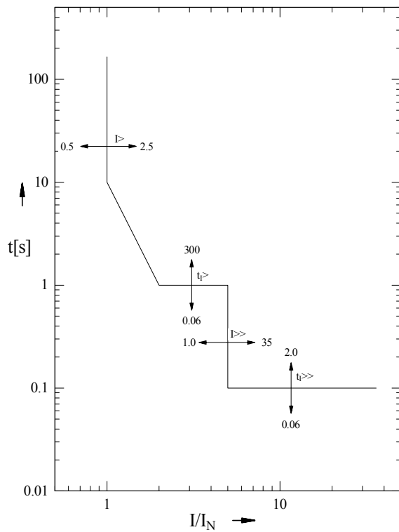
Figure 7.12: Setting example: Overcurrent setting with short circuit function and limiting the tripping characteristic
