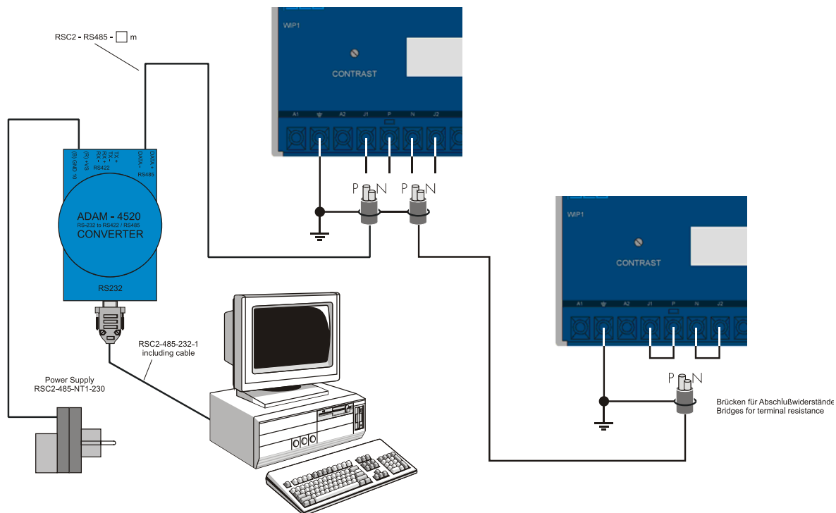
Figure 3.6: Connection of the serial interface
