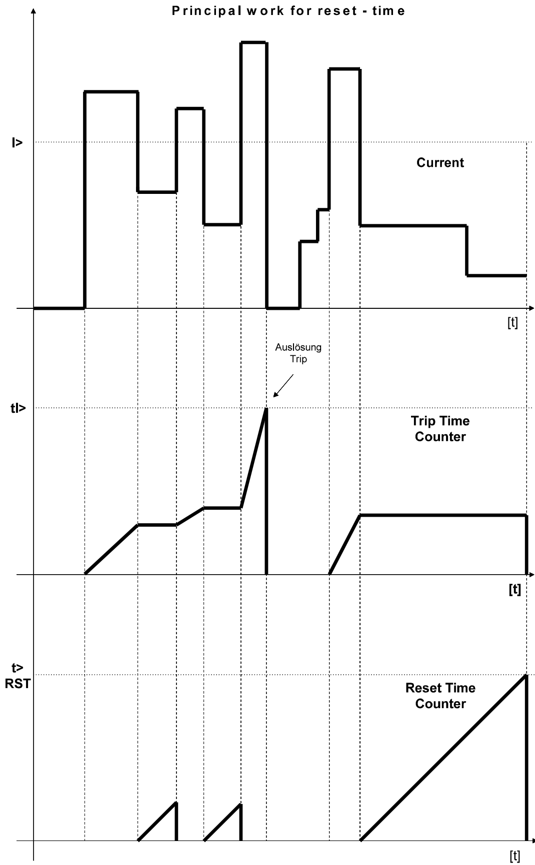
Figure 7.13: Trip example
