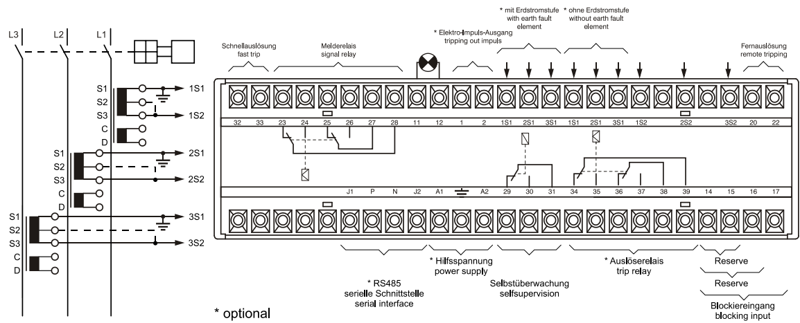
Figure 3.1: Connection example with relay tripping
