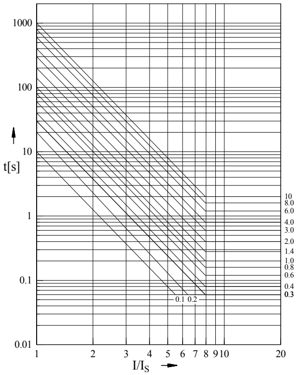
Figure 7.9: x^3 - tripping characteristic
