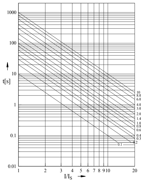
Figure 7.7: x^2 - tripping characteristic
