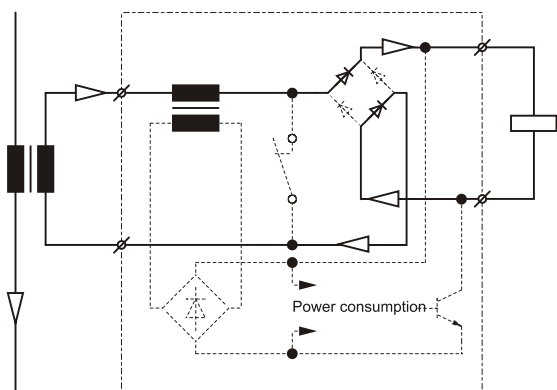
Figure 4.3: Tripping via current transformer I < 12 \times I_n
