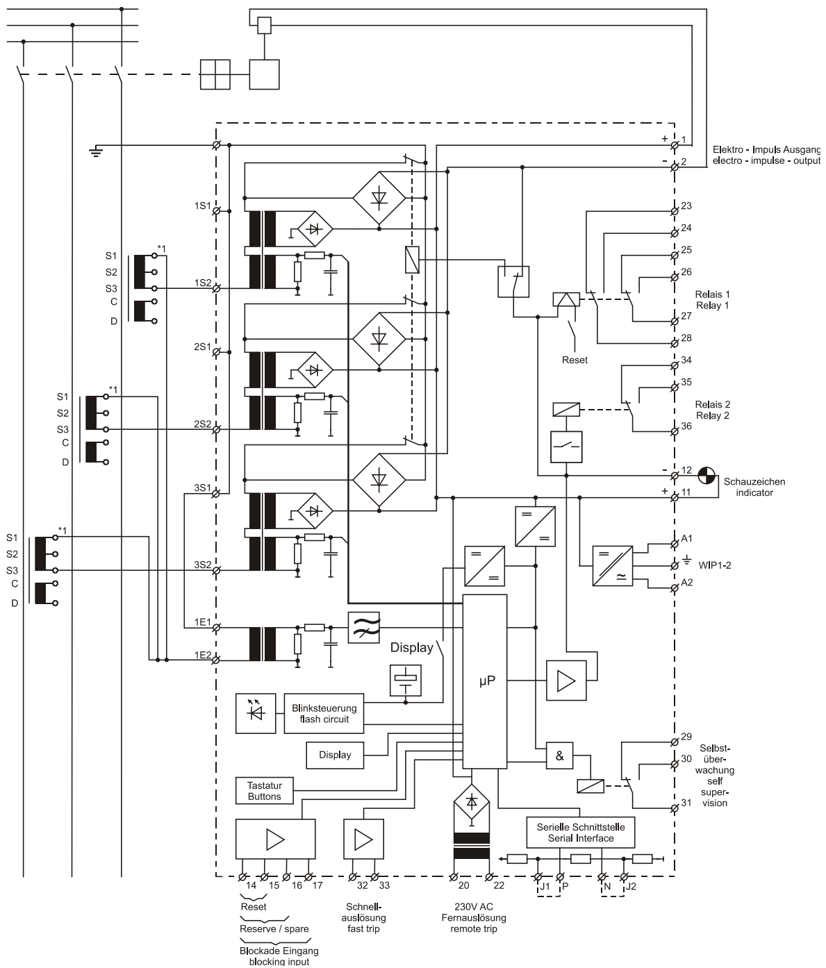
Figure 3.2: Block diagram
