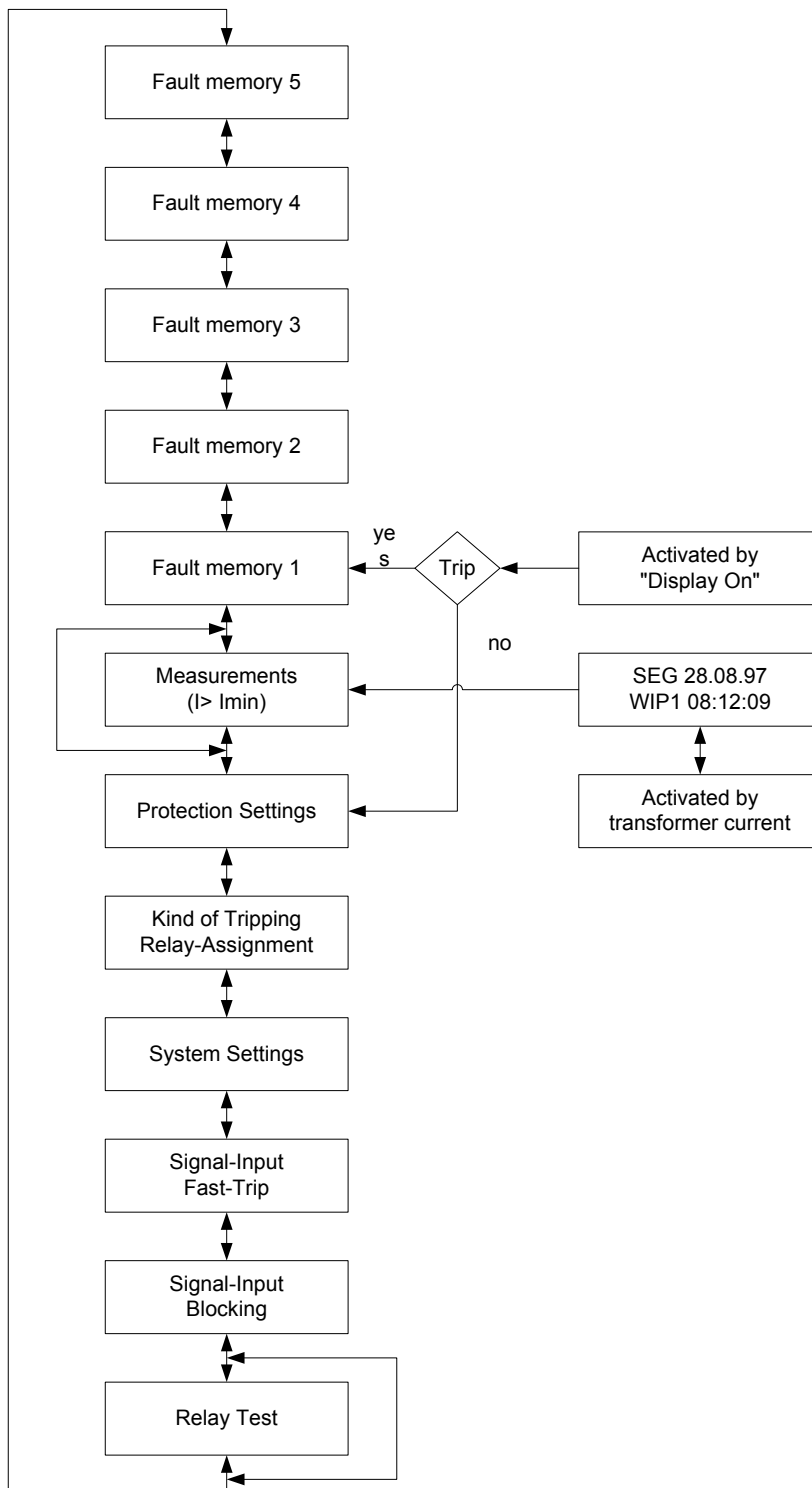
Figure 5.1: Main menu overview
