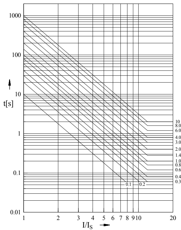
Figure 7.8: x^{2.5} - tripping characteristic
