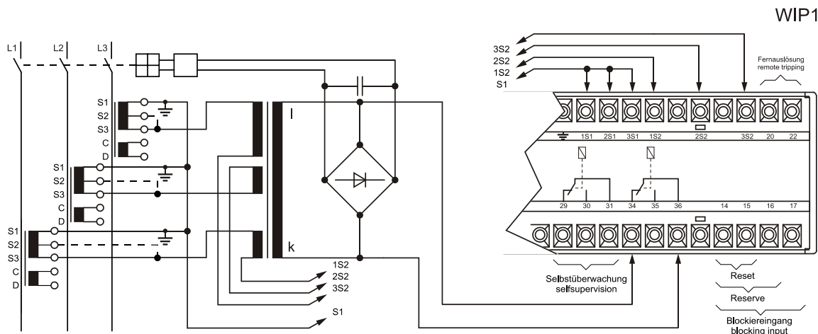
Figure 3.5: Connection example with relay tripping
