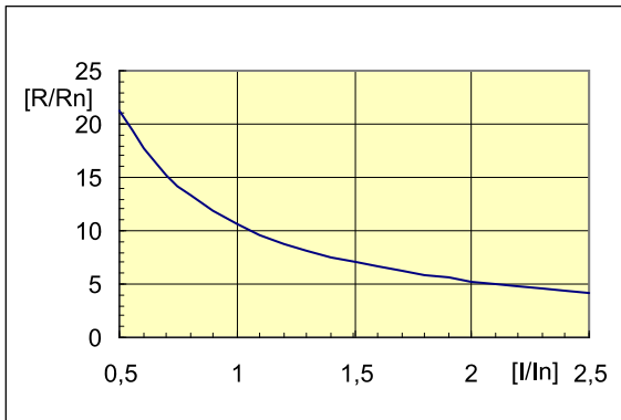
Figure 4.5: Minimum coil resistance
